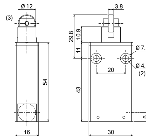
03 90° roller plunger
